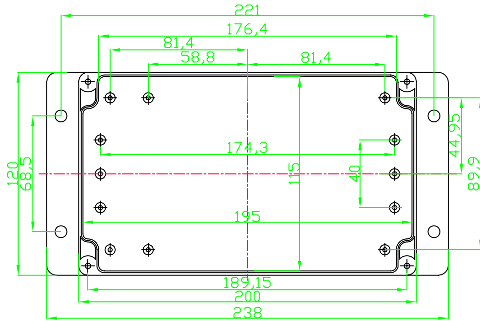
HOUSING
